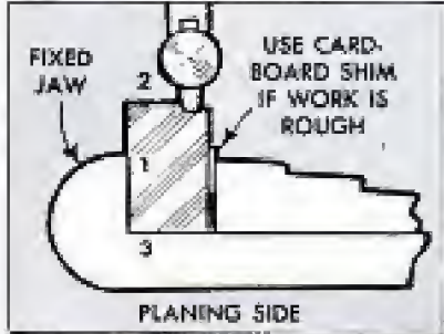
8 PLANING SIDE No. 2
